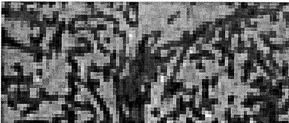
Figure 3. Tomographic "slice" through a vertical plane of a papermaker's felt. The reorientation of fibers due to a needle penetration can be seen in the center of the image.
