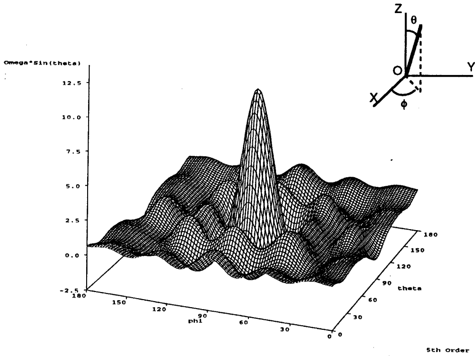
Figure 2: Orientation Distribution Function of Model I
