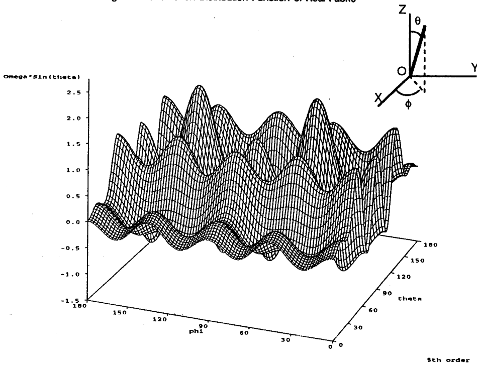
Figure 4: Orientation Distribution Function of Real Fabric
