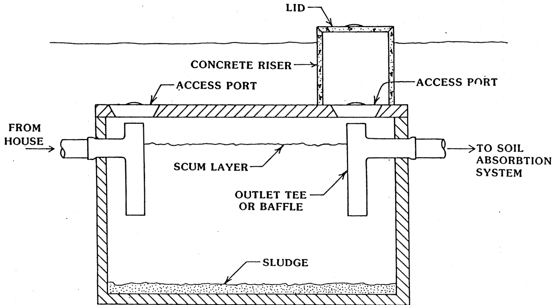
FIG. 1 TYPICAL DOMESTIC SEPTIC TANK
