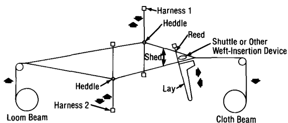
Elements of the Loom
