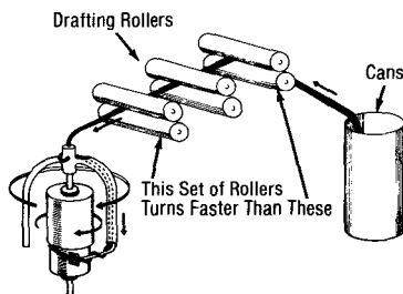
The Roving Operation
