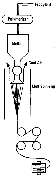
Polypropylene Fiber Production
