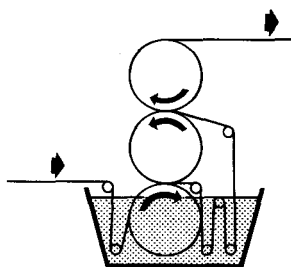
Double-Dip, Double-Nip Padding
