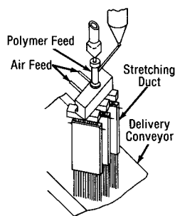
Spunbonding: Polymer-to-Web System
