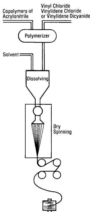
Modacrylic Fiber Production
