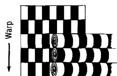
A Corded Effect Running in the Filling Direction
