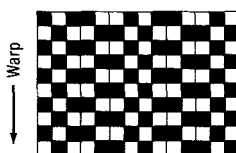
A Corded Effect Running in the Warp Direction
