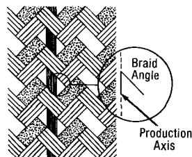
Braided Fabric Showing Braid Angle
