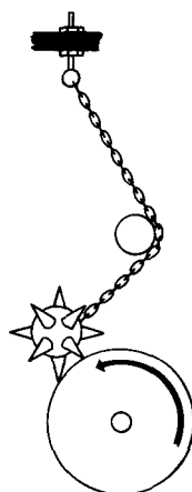
Mace Snag Tester
