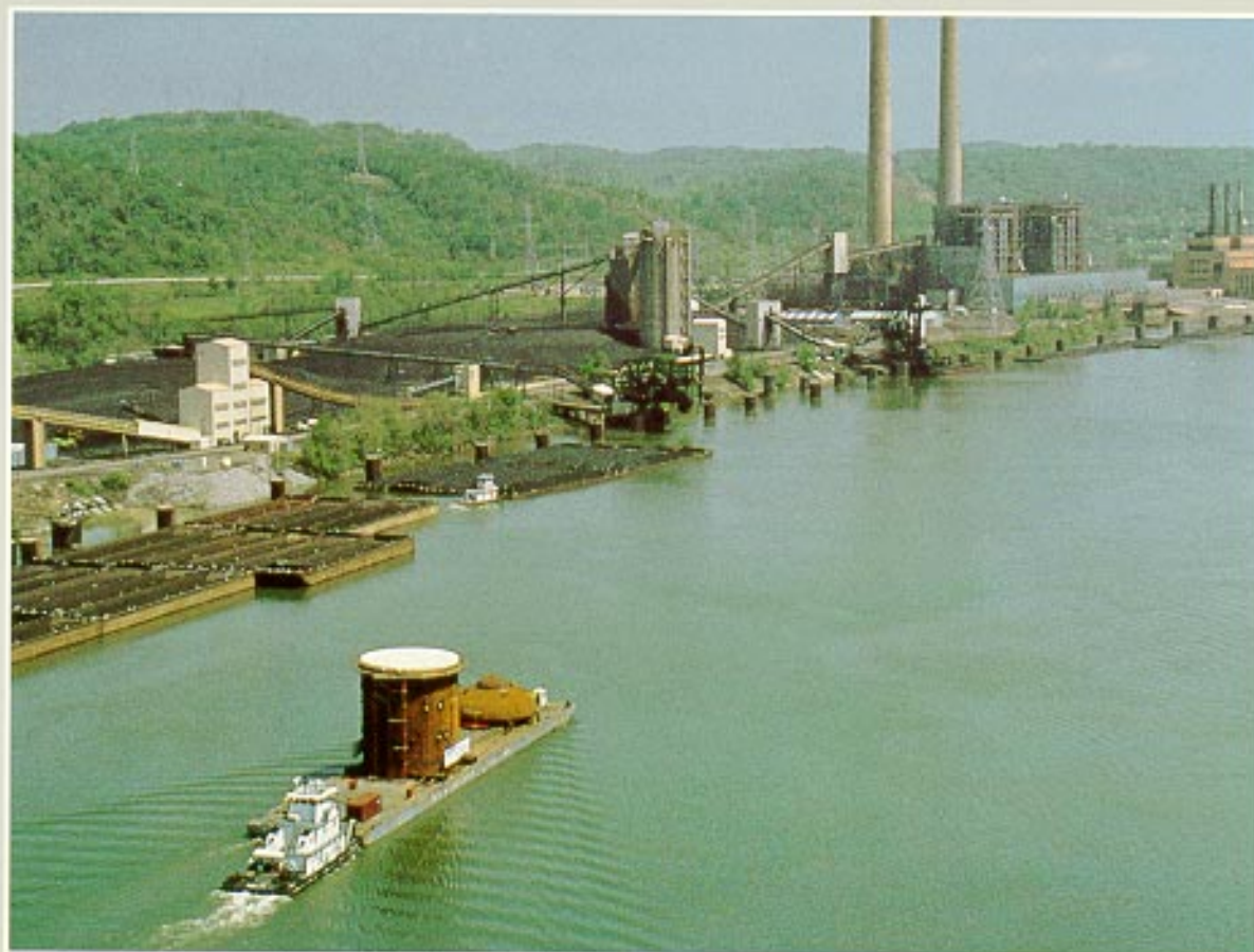
Tidd: The Nation's First PFBC Combined-Cycle Demonstration
