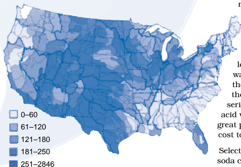
Figure 1: Average Water Hardness in the Continental United States
