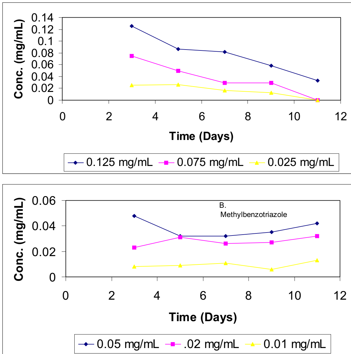
Figure 1. Degradation of benzotriazoles added to fungal cultures after induction with veratryl alcohol.
