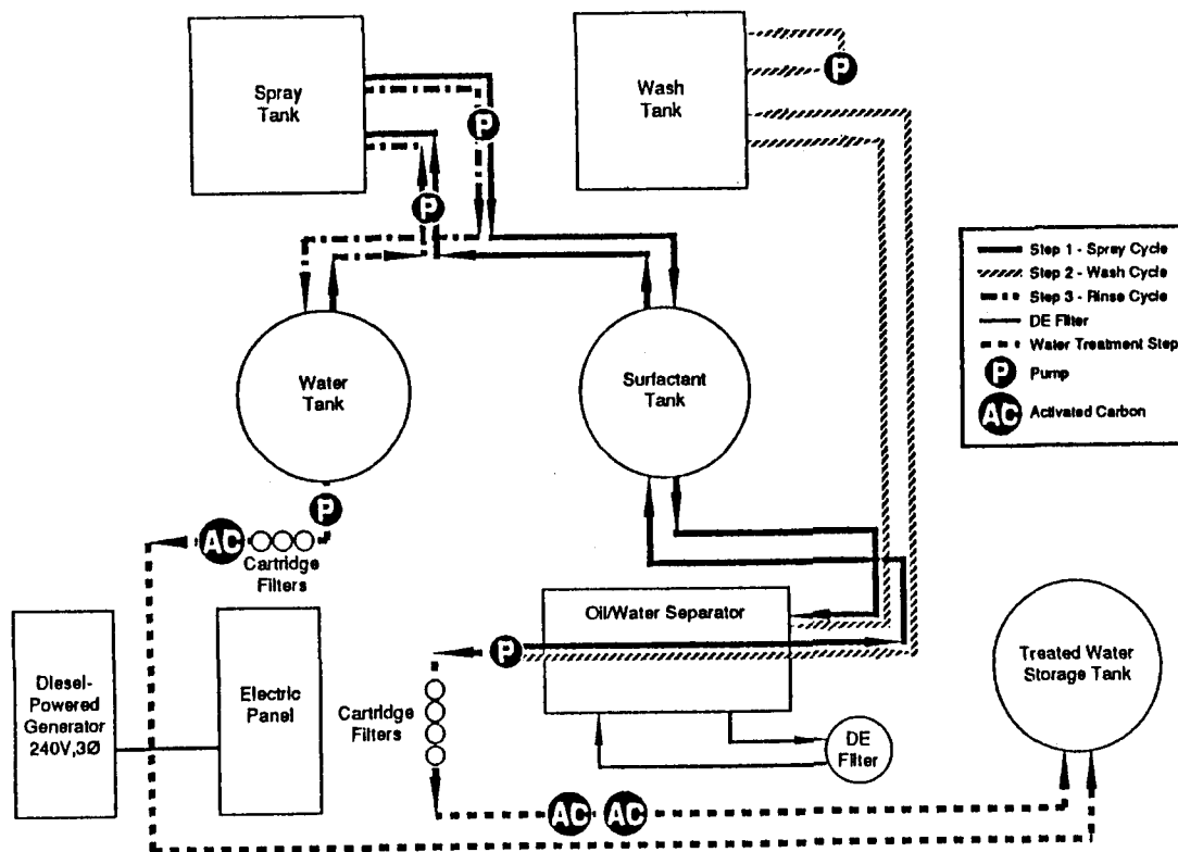
Figure 1. Schematic of Pilot - Scale Debris Washing System.
