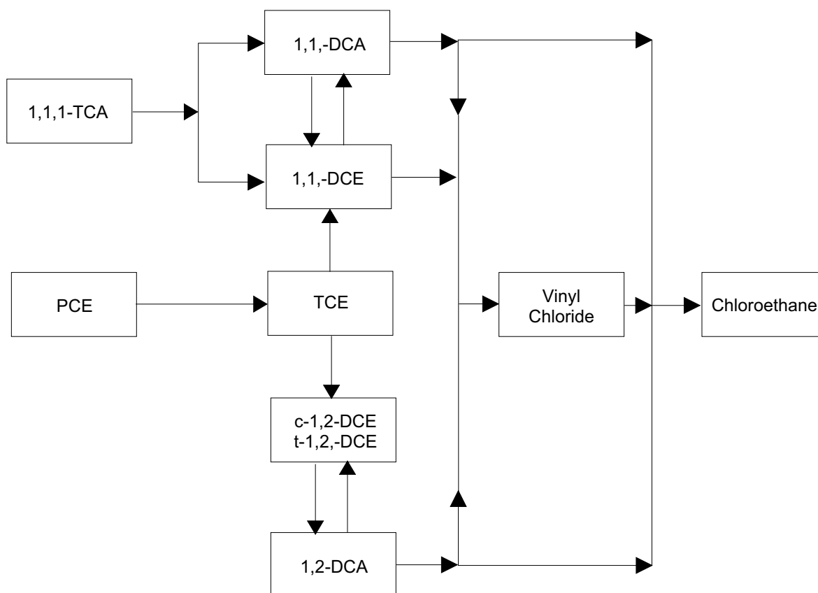
Figure 2. Transformation pathways for various chlorinated volatile hydrocarbons in soil systems (Dragun 1988).
