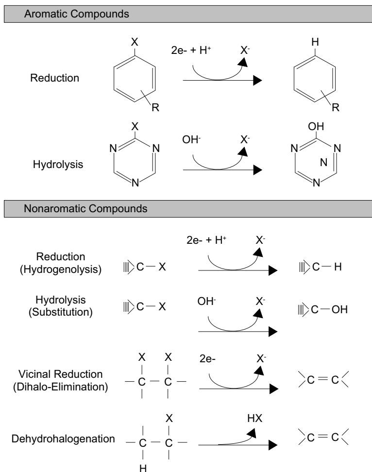
Figure 1. Examples of anaerobic dehalogenation mechanisms for aromatic and nonaromatic pesticides (Kuhn and Suflita, 1989a)
