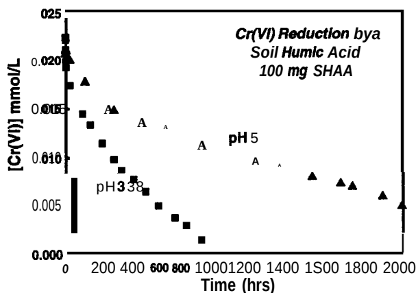
Figure 4. Reduction of \text{Cr(VI)} in a suspension of 100 mg/L soil humic acid (SHA) at pH 3 and 5 (Wittbrodt and Palmer, in preparation).
