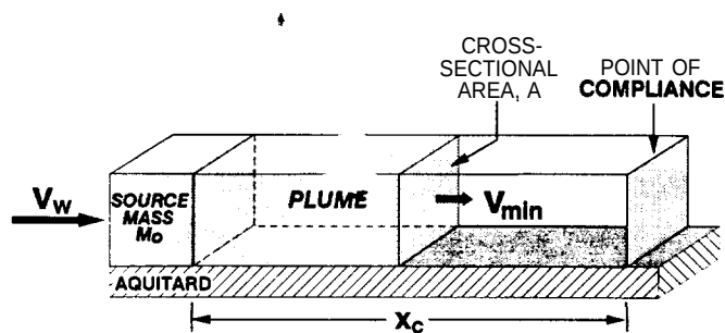
Figure 6. Cr-plume moving from the source area to the point of compliance. The initial Cr(VI) concentration in the source area is M_0 , v_w is the groundwater velocity, v_{\min} is the velocity of the Cr(VI) front assuming instantaneous reduction of the Cr(VI), and X_c is the distance from the source area to the point of compliance.
