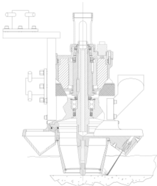
Figure 3. Schematic of the CSEE.
