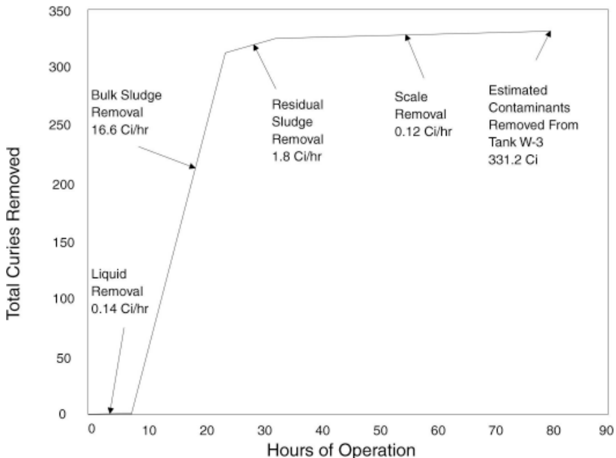
Figure 8. Summary of Tank W-3 cleaning efficiency.
