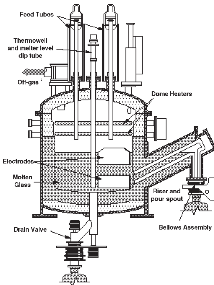
Figure 2. Joule-heated melter.
