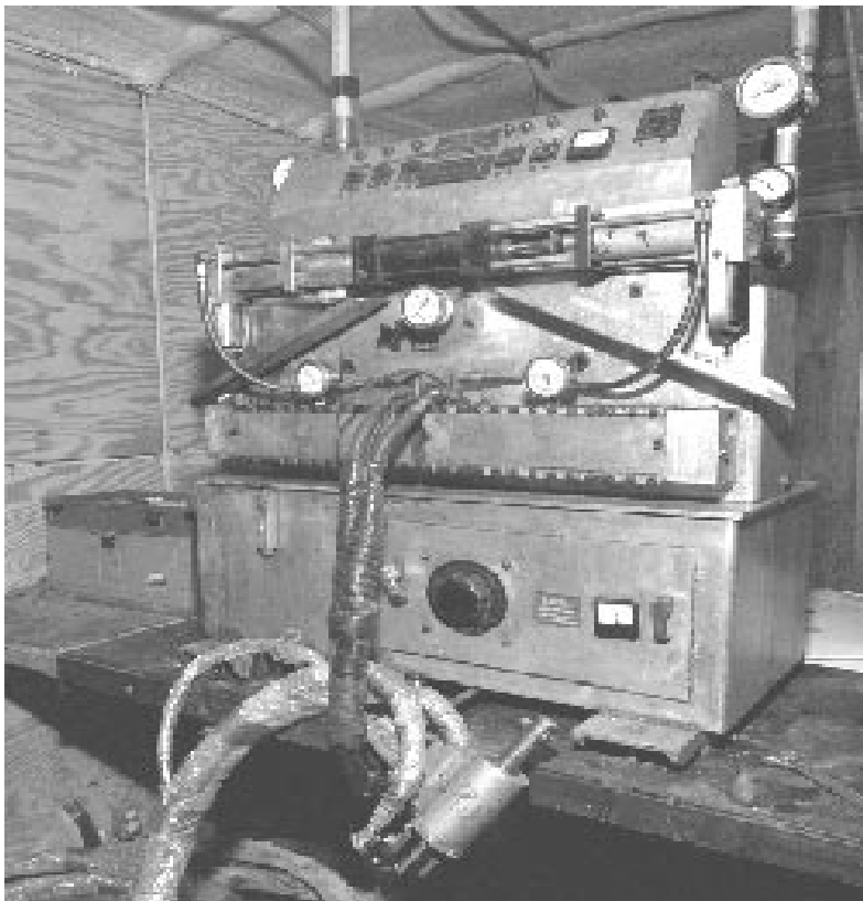
Figure 1. The mixing control unit regulates and pumps chemicals to the mixing gun.
