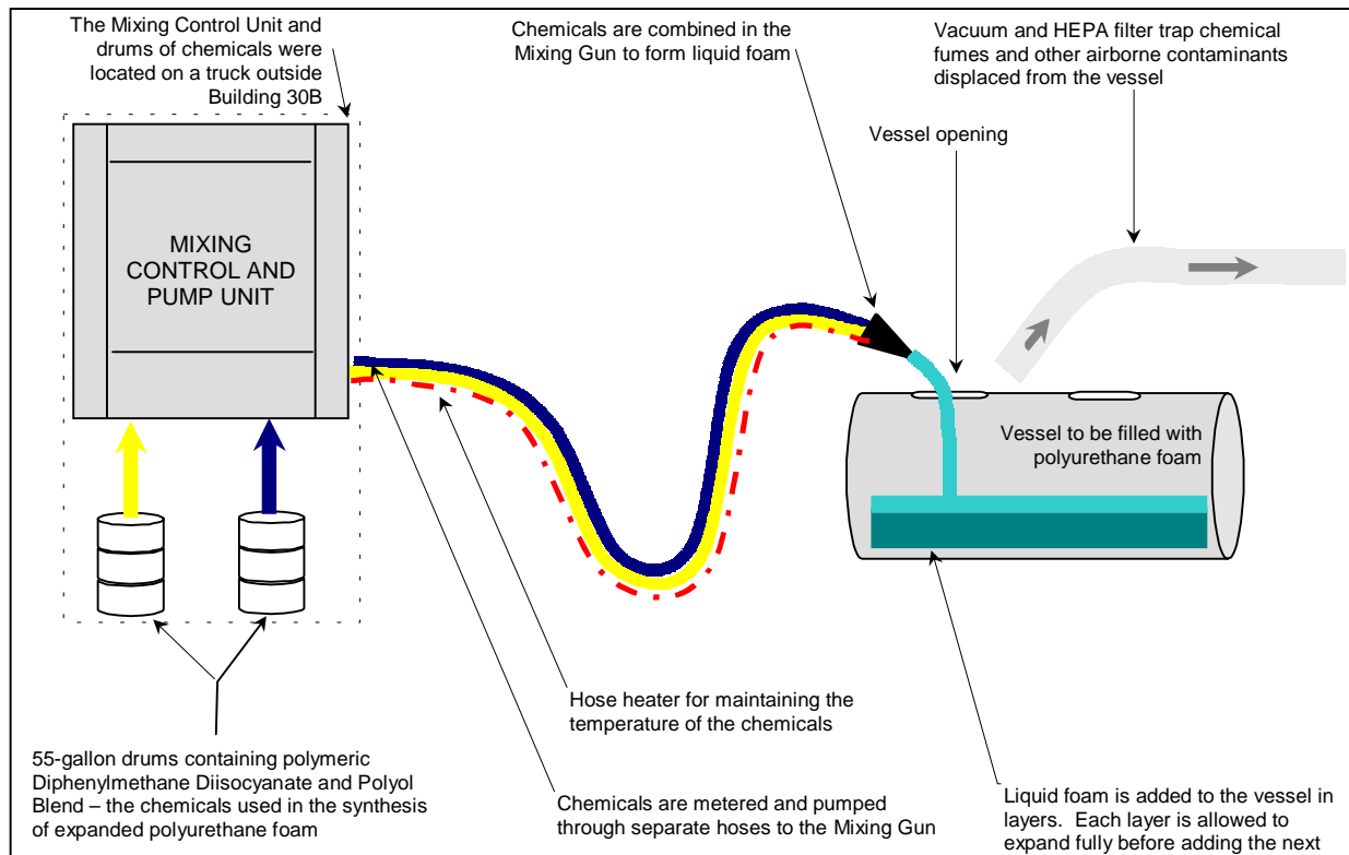
Figure 3. Schematic of the expanded polyurethane foam void filling process.
