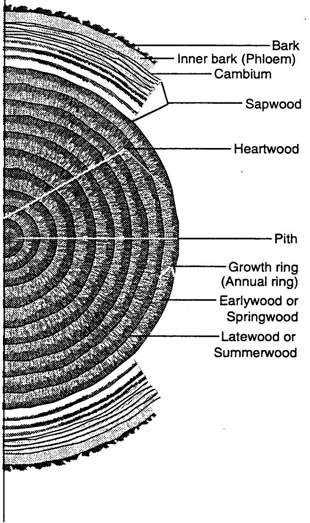
Figure 1.2 Principle features of a tree stem, cross-sectional (transverse) view.
