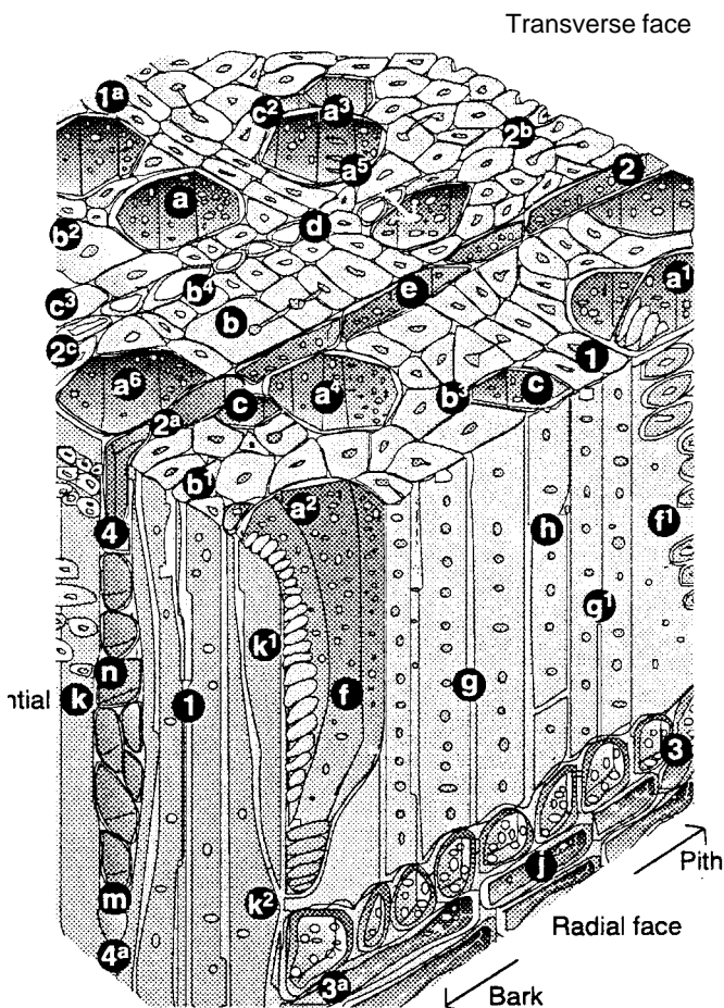
Figure 1.5 Schematic drawing of a typical hardwood-sweetgum. (magnified 330X)
