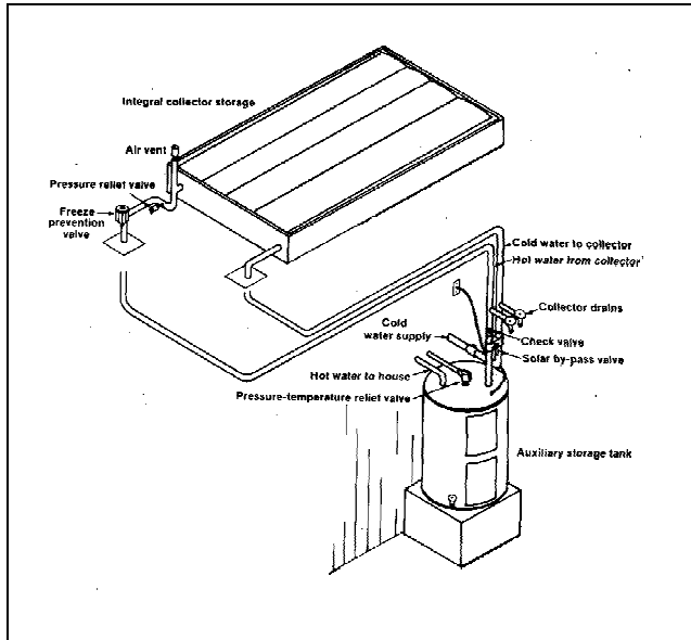
Figure 6. Integral collector storage system.
