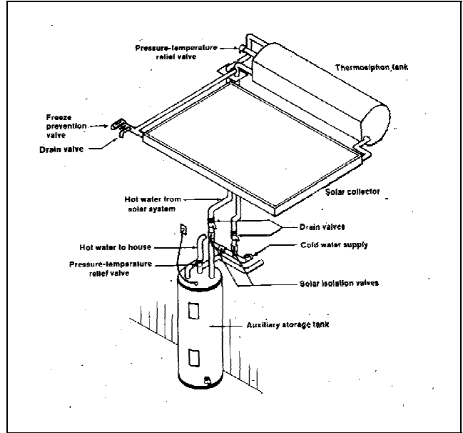
Figure 5. Thermosiphon system.
