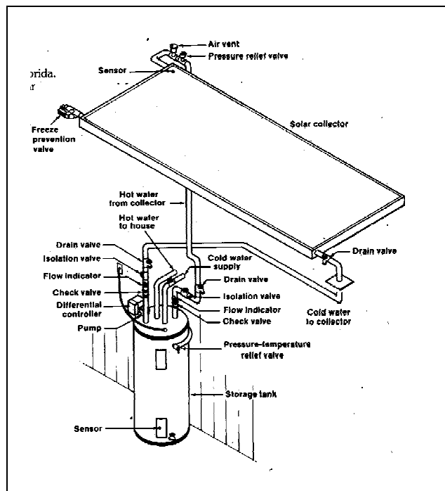
Figure 1. Typical direct pumped system.
