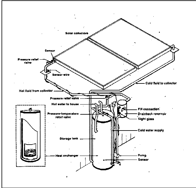
Figure 4. Indirect system using distilled water.
