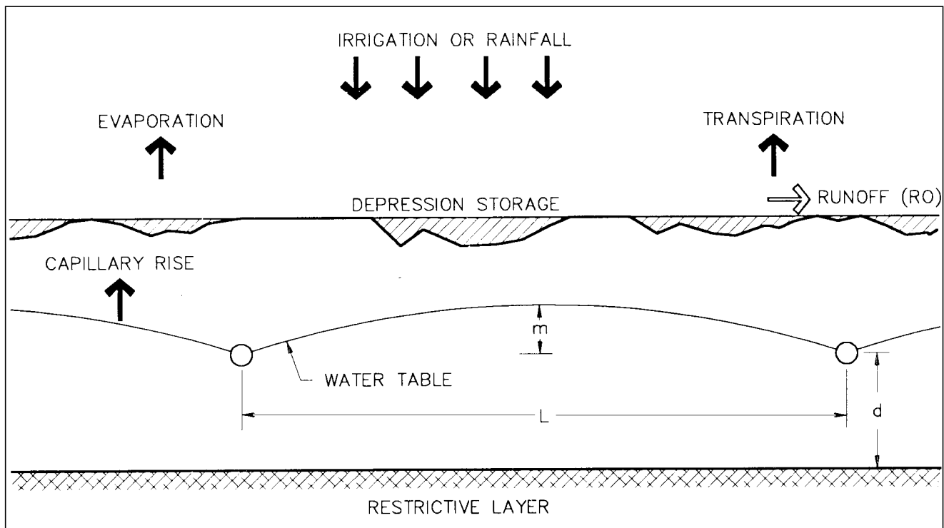
Figure 2. A subsurface drainage system. Plastic draitubes are located a distance ( L ) apart.
