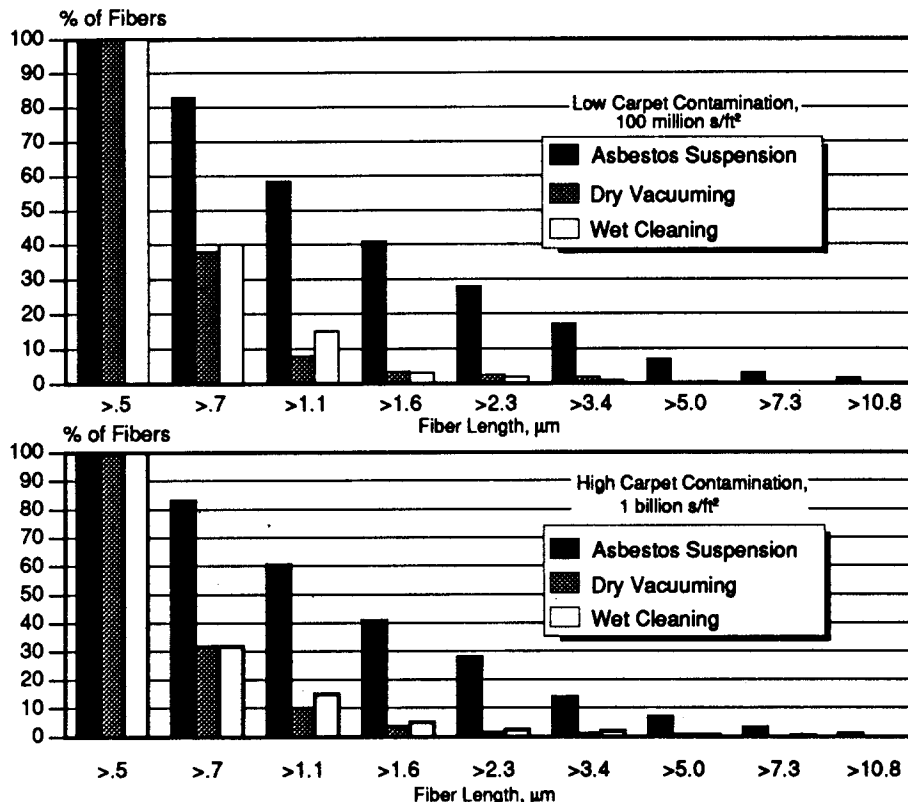
Figure 2. Comparative plot of cumulative percentages of airborne asbestos fibers during dry vacuuming and wet cleaning of carpet with asbestos fibers in the low and high concentration suspensions.
