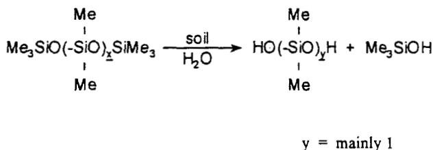
Fig. 4. Degradation of PDMS during soil contact to form siloxanols and silanols.
