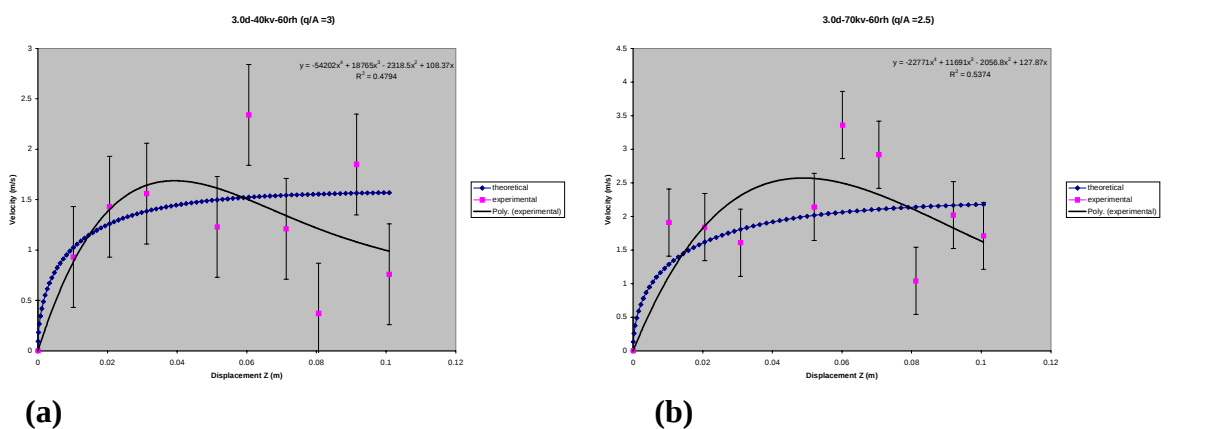
Figure 7. Velocity Profile for 3d-2.5mm Flocks at 60 % RH. (a) 40 kV, (b) 70 kV.
