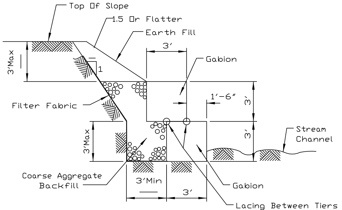
SECTION
