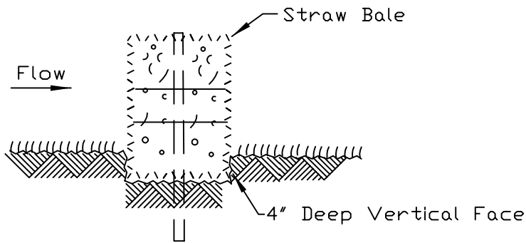
BEDDING DETAIL
