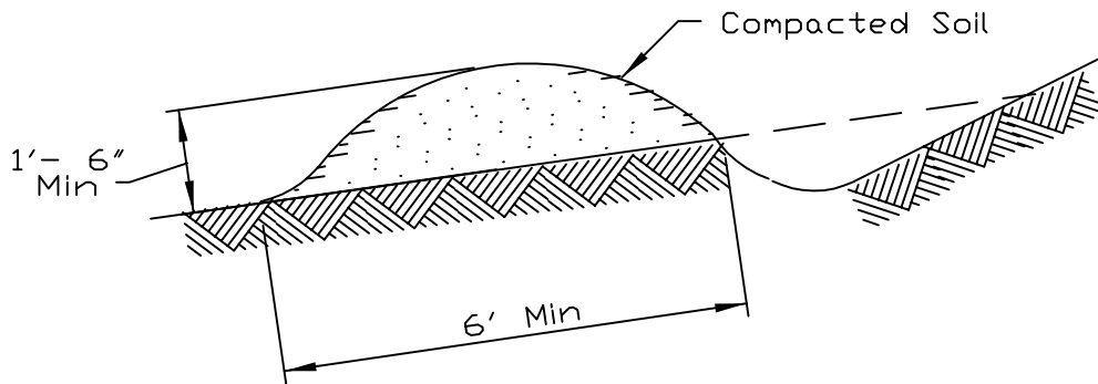
TYPICAL EARTHEN STRUCTURE
