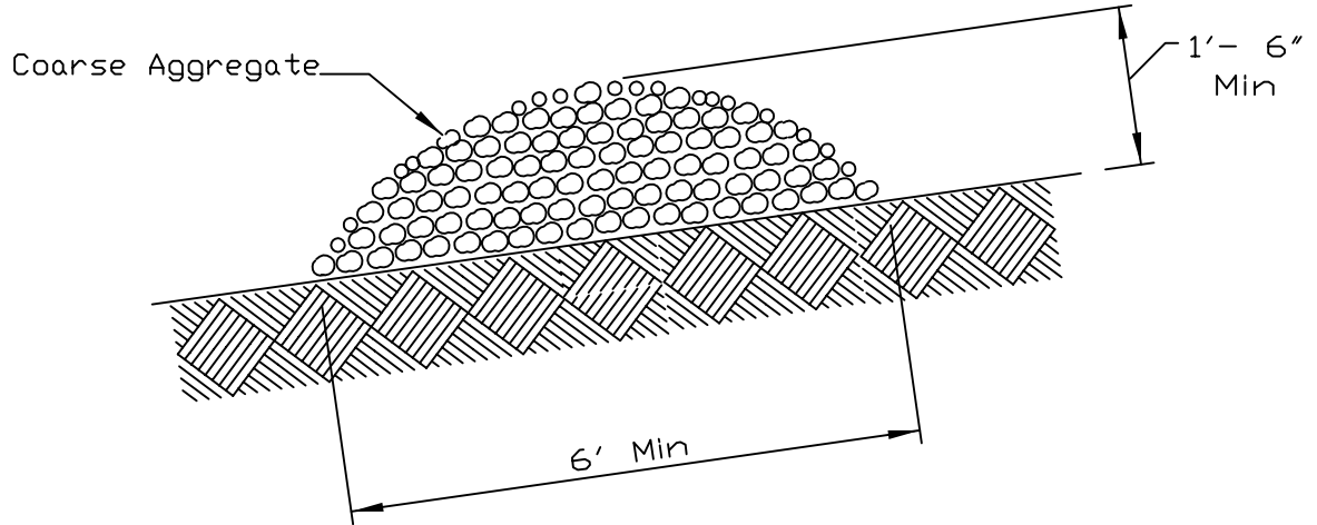
TYPICAL GRAVEL STRUCTURE
