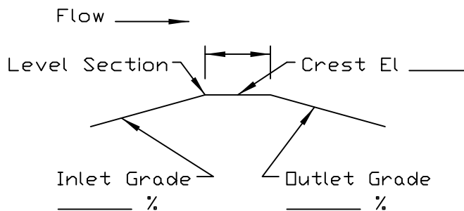
PROFILE ON CENTERLINE OF EMERGENCY SPILLWAY
