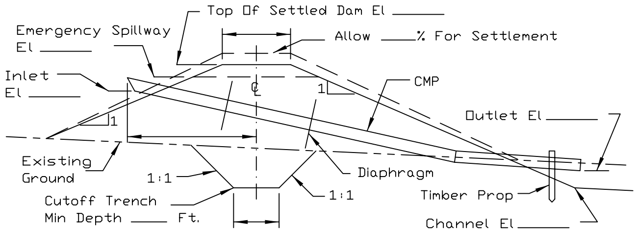
MAXIMUM CROSS SECTION OF DAM
