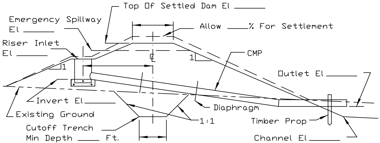
MAXIMUM CROSS SECTION OF DAM
