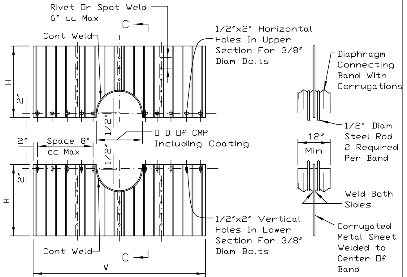
DETAILS OF ANNULAR PIPE DIAPHRAGMS
