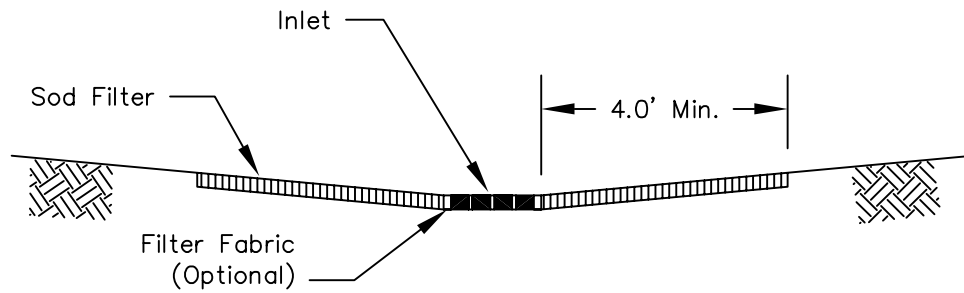
SECTION
