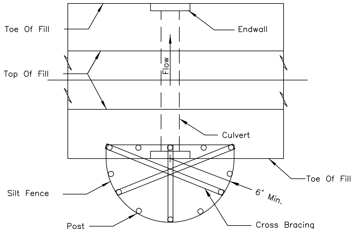
PLAN VIEW
